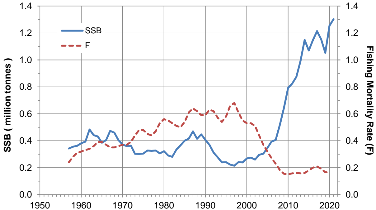
Figure 5 The spawning stock biomass (SSB) of North Sea plaice from 1957 to 2021 with the projected SSB in 2022, and the fishing mortality rate ( F ) from 1957 to 2020 with the projected F in 2021. (ICES Data; see p. 2.)
