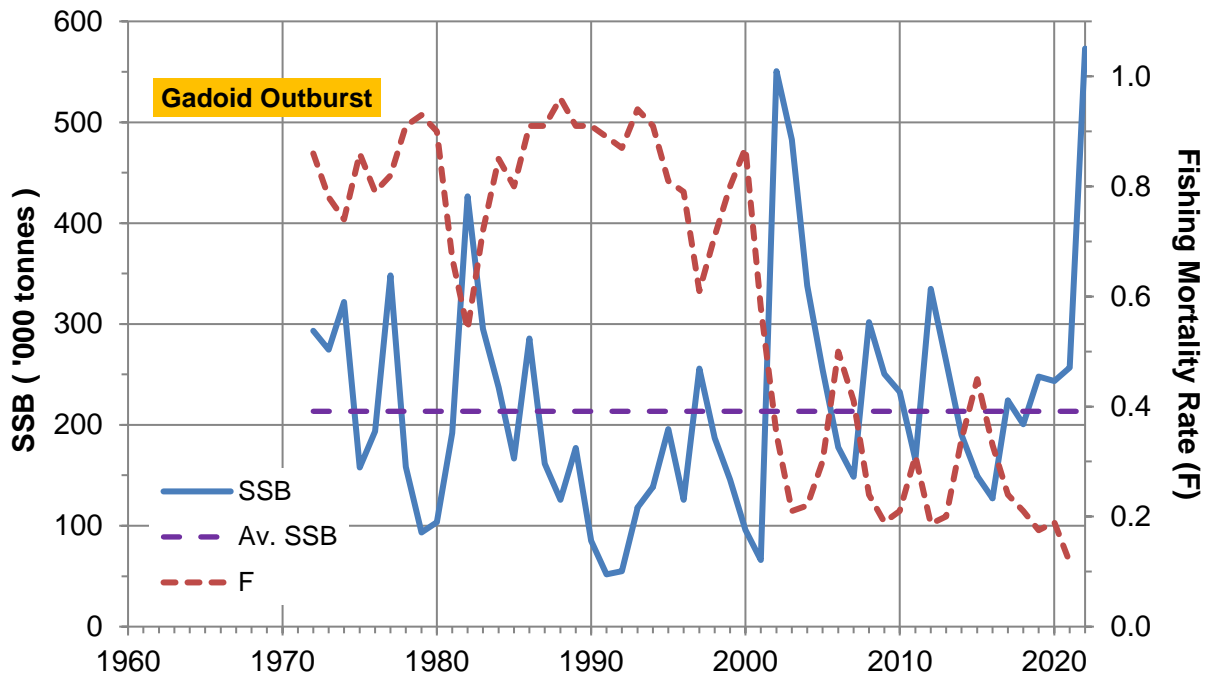
Figure 2 The spawning stock biomass (SSB) of the combined North Sea and West of Scotland haddock from 1972 to 2021 with the projected SSB in 2022, and the fishing mortality rate ( F ) from 1972 to 2020 with the projected F in 2021. The horizontal dashed line shows the average SSB over the whole time-series (1972 – 2021). In the 1960s and 1970s the abundance of haddock was enhanced by the 'gadoid outburst' (see p. 3). (ICES Data; see p. 2.)
