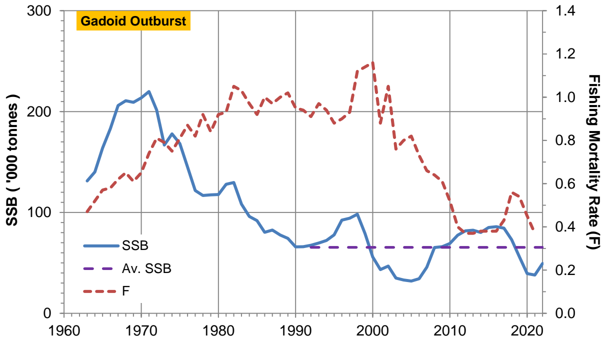
Figure 1 The spawning stock biomass (SSB) of North Sea cod from 1963 to 2021 with the projected SSB in 2022, and the fishing mortality rate ( F ) from 1963 to 2020 with the projected F in 2021. The horizontal dashed line shows the average SSB over the last 30 years (1992 – 2021). In the 1960s and 1970s the abundance of cod was enhanced by the ‘gadoid outburst’ (see p. 3). (ICES Data; see p. 2.)
