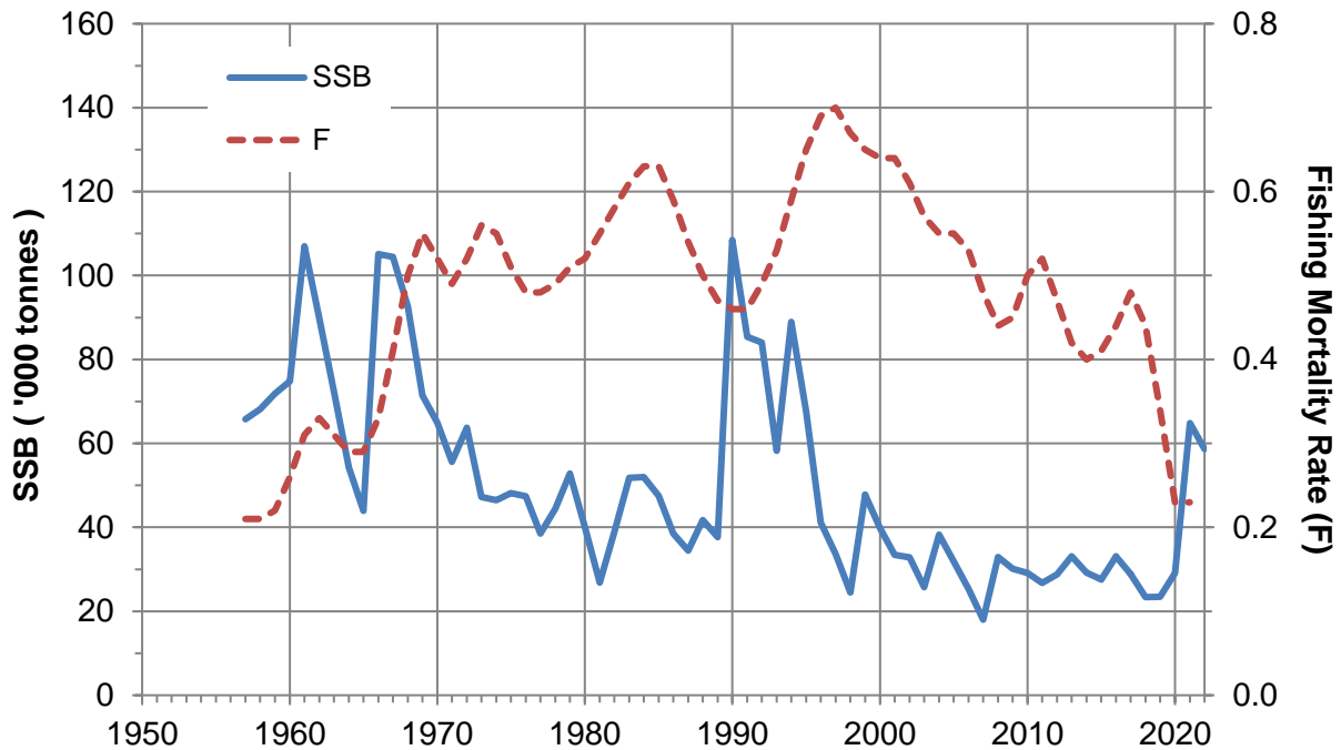
Figure 6 The spawning stock biomass (SSB) of North Sea common sole (Dover sole) from 1957 to 2021 with the projected SSB in 2022, and the fishing mortality rate ( F ) from 1957 to 2020 with the projected F in 2021. (ICES Data; see p. 2.)
