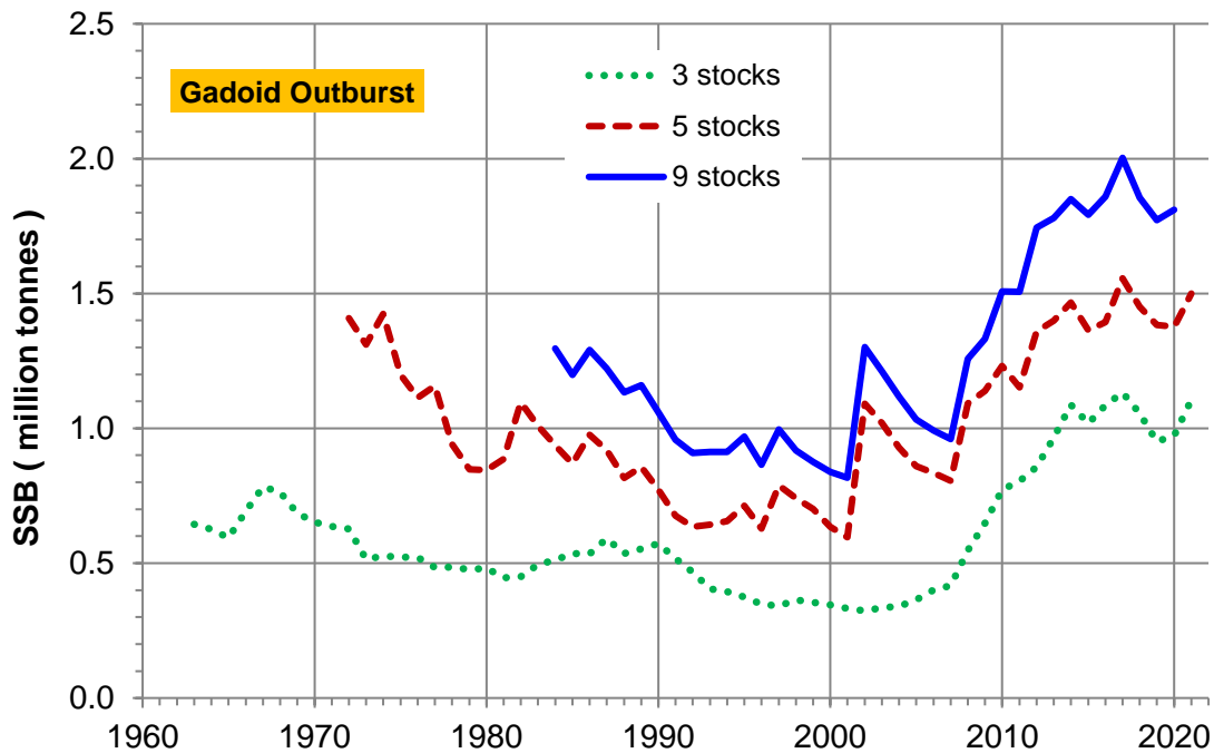
Figure 11 The total combined spawning stock biomasses (SSB) of three, five and nine fish stocks for which long-term time-series are available (see table below for stocks). (Based on analysis of ICES Data; see p. 2.)
