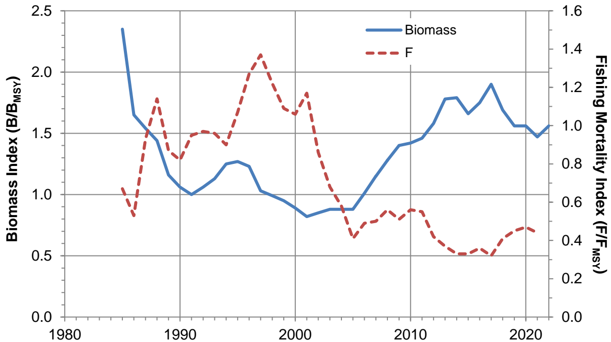
Figure 8 The index of the biomass ( B ) of the North Sea and West of Scotland megrim stock from 1985 to 2021 with the projected index in 2022, and the index of the fishing mortality rate ( F ) from 1985 to 2020 with the projected index in 2021. (ICES Data; see p. 2.)
