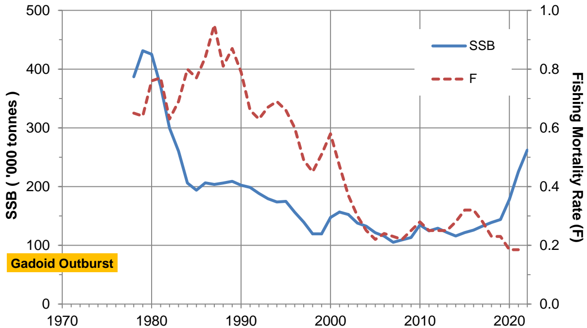
Figure 4 The spawning stock biomass (SSB) of North Sea whiting from 1978 to 2021 with the projected SSB in 2022, and the fishing mortality rate ( F ) from 1978 to 2020 with the projected F in 2021. In the 1960s and 1970s the abundance of whiting was enhanced by the 'gadoid outburst' (see p. 3). (ICES Data; see p. 2.)
