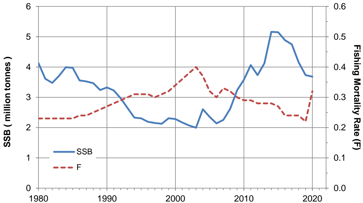
Figure 14 The spawning stock biomass (SSB) of the North-East Atlantic mackerel stock* from 1980 to 2019 and the projected SSB in 2020, and the fishing mortality rate ( F ) from 1980 to 2019 and the projected F in 2020. (ICES Data; see p. 2.)
