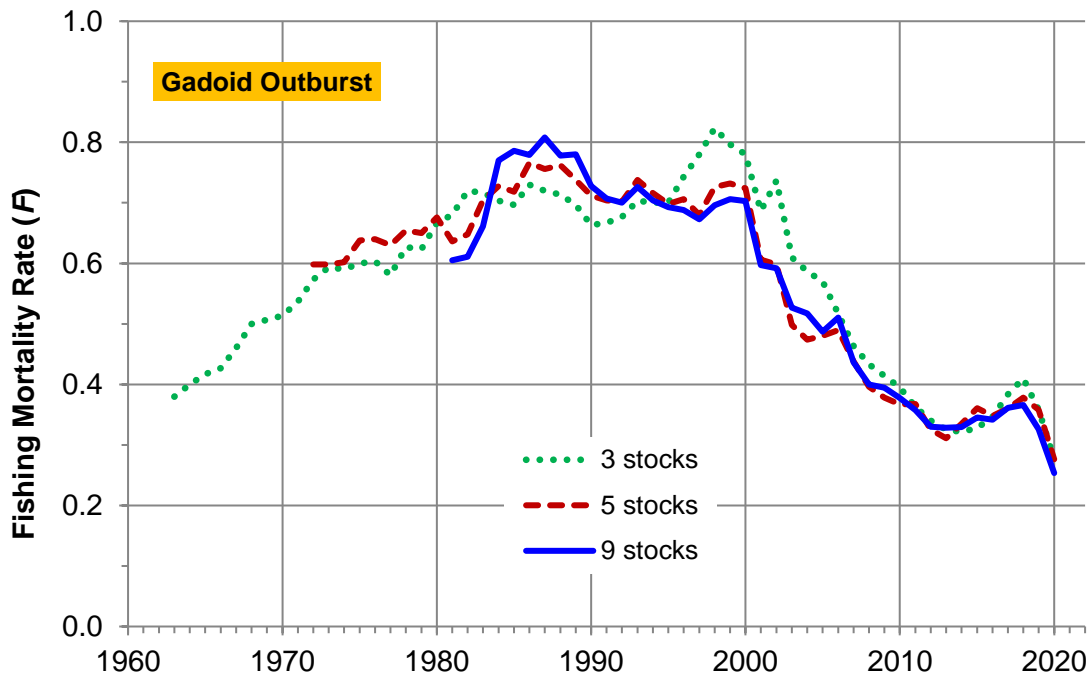
Figure 12 The overall average fishing mortality rate ( F ) of three, five and nine fish stocks for which long-term time-series are available (see table below for stocks). (Based on analysis of ICES Data; see p. 2.)
